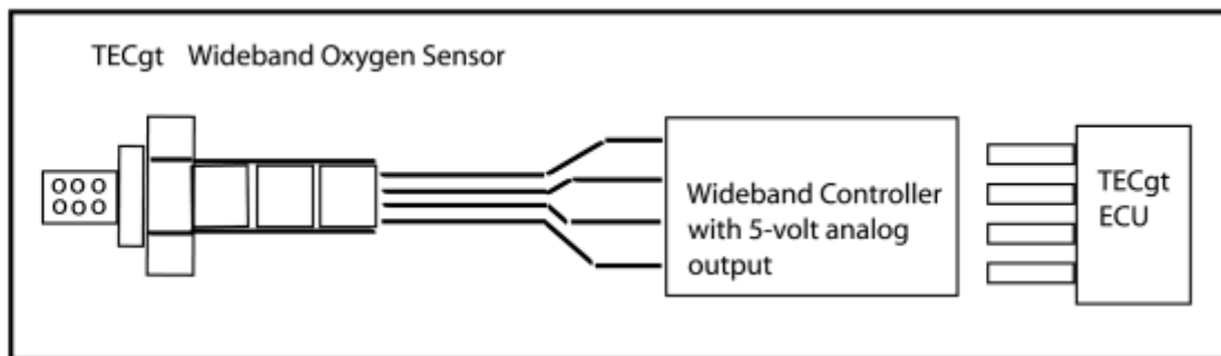
Figure 57- Typical Wideband Configuration
