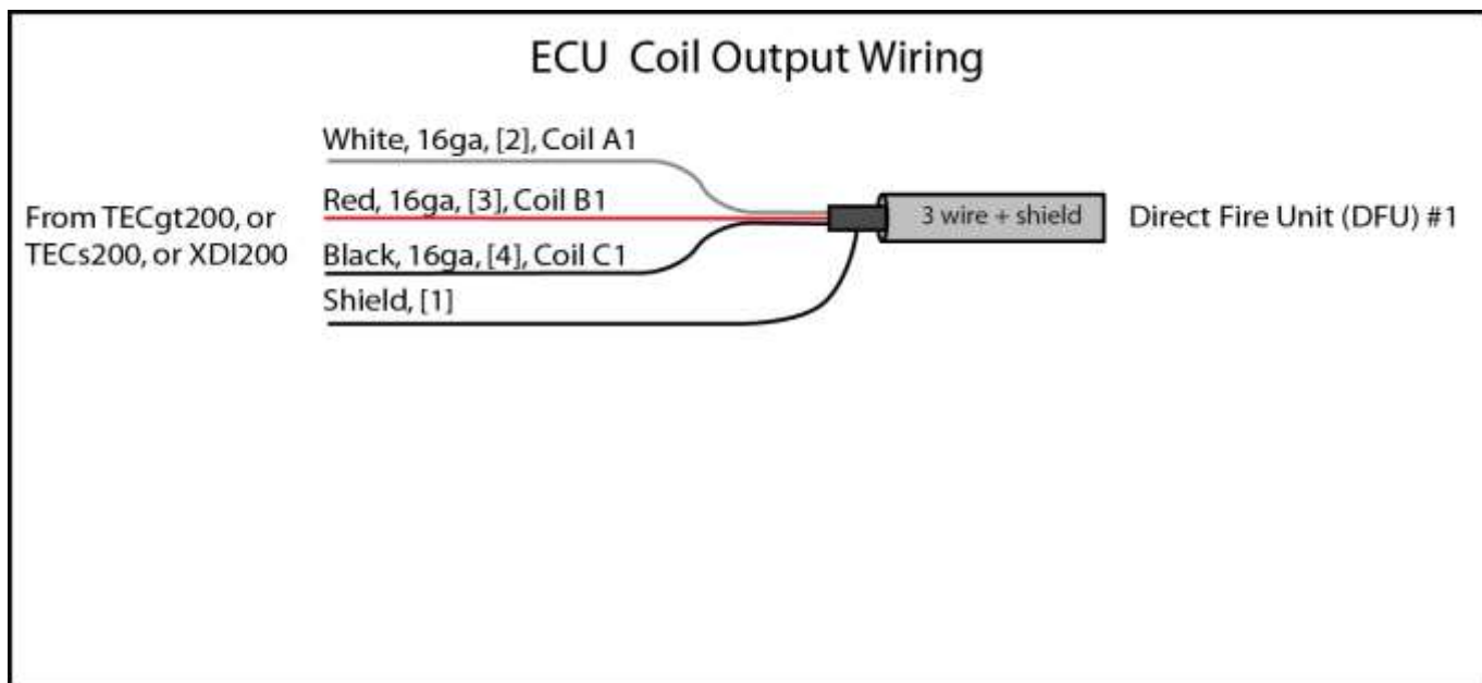
Figure 25: ECU Coil Output Wires (note: shield wire is connected inside the TECs200 unit, not connected at the coils).
