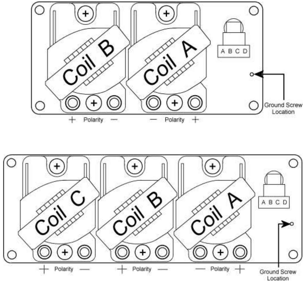
Figure 120: DFU Secondary Voltage Polarity – for Redundant Ignition Applications.
