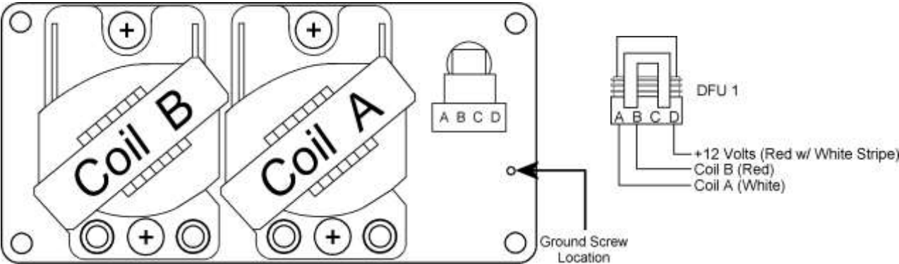
Figure 27. 4-Cyl DFU Setup
