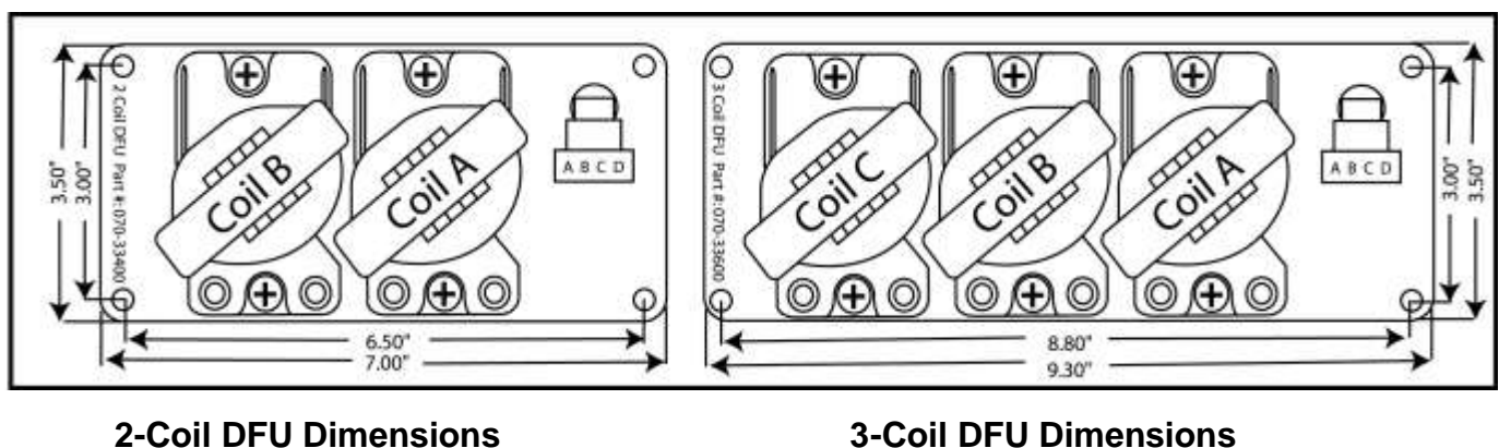
Figure 1. Electromotive Direct Fire Units
