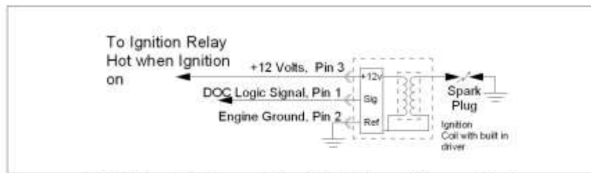
3 Wire Driver On Coil Ignition Coil (Example shown is Hitachi, Honda coil)
