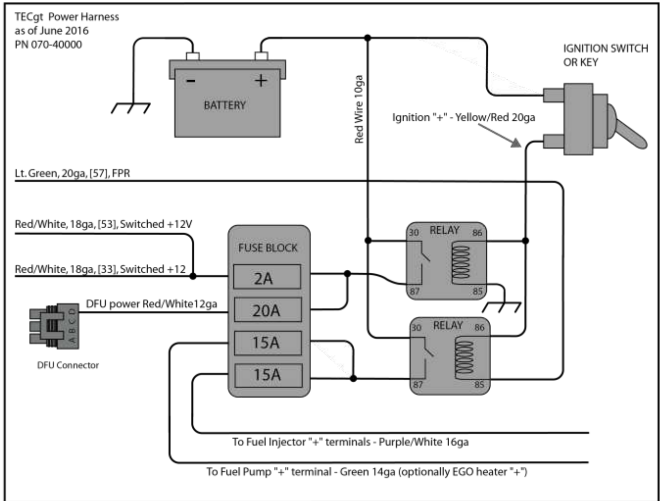
Figure 15. TECgt200 Power Harness (PN: 070-40000).
