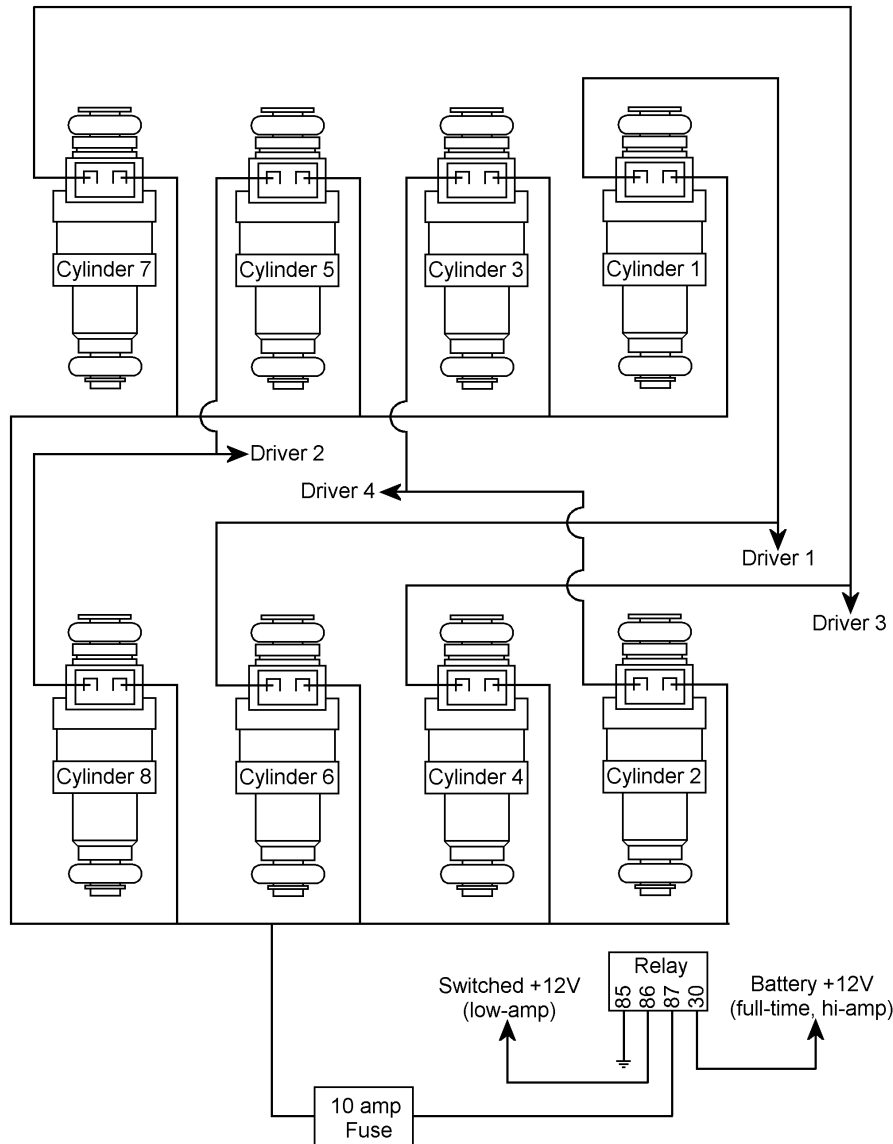
Figure 20: 8-cylinder phase-sequential injector wiring for firing order 1-8-4-3-6-5-7-2.
