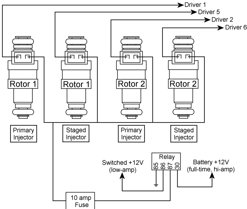
Figure 22 Rotary injector wiring.
