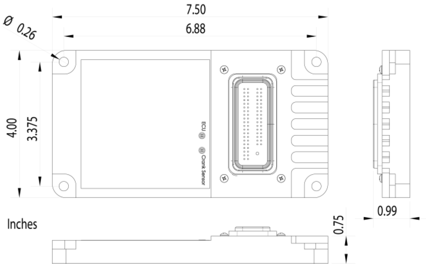
Figure 2. TECgt200 ECU
