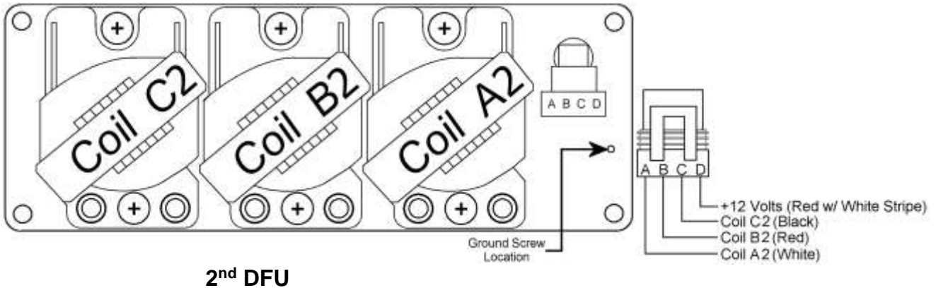
Figure 30: (The above picture is from a twin-plug 6 Cyl.), if running a V8 the first DFU will have coils A1, B1 the second DFU will have coils A2, B2.
