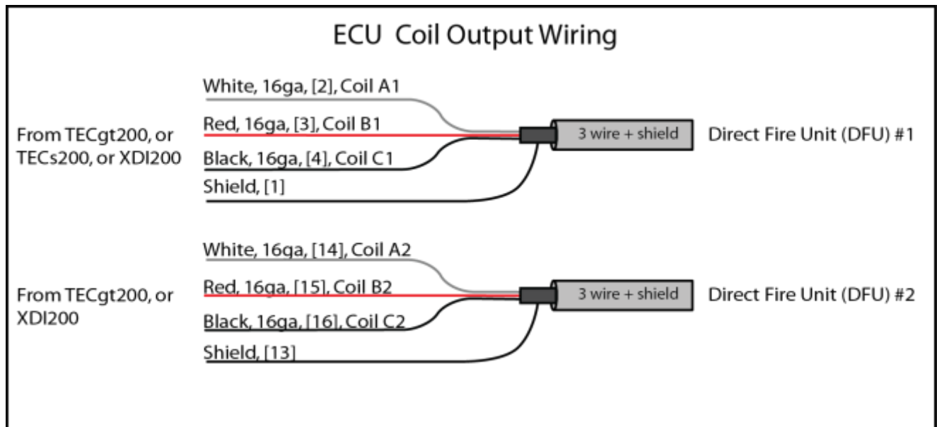
Figure 25: ECU Coil Output Wires (note: shield wire is connected inside the TECgt200 unit, not connected at the coils).
