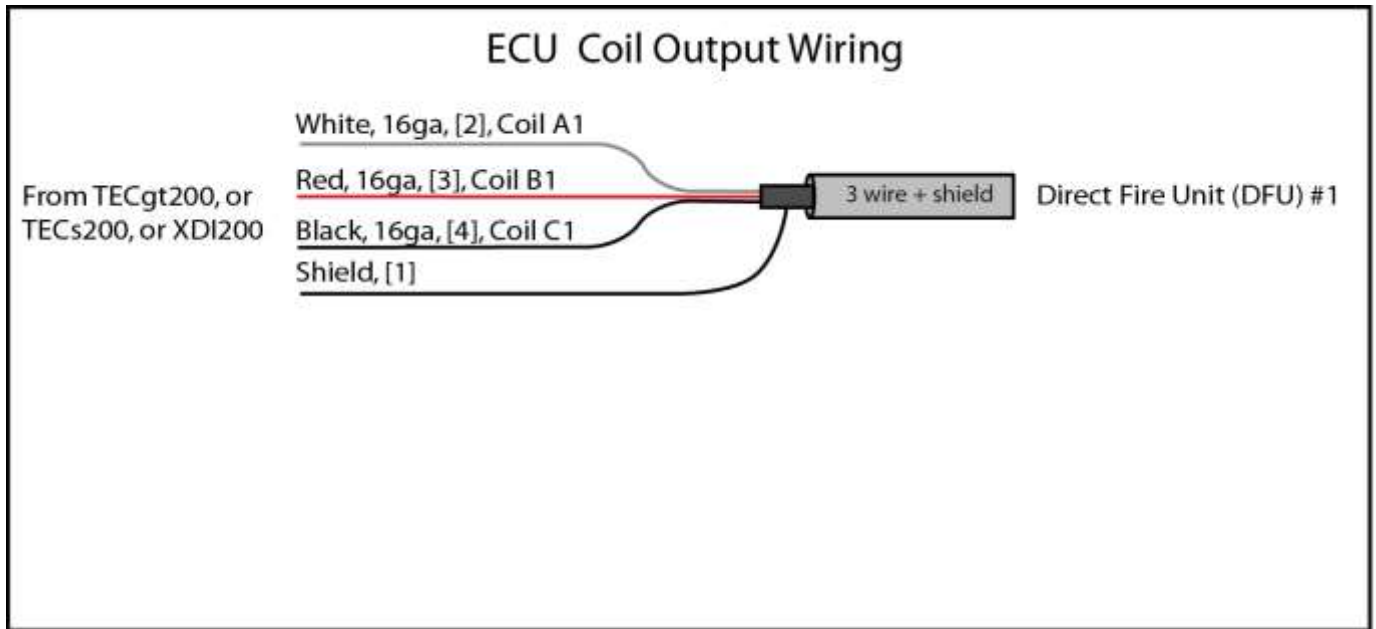
Figure 25: ECU Coil Output Wires (note: shield wire is connected inside the TECs200 unit, not connected at the coils).
