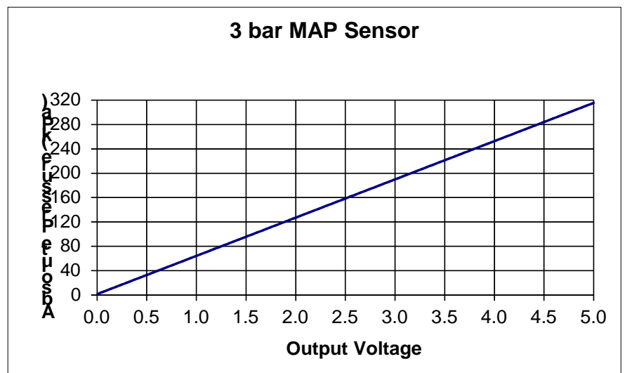
Figure 108: 3-Bar MAP sensor output voltage.
