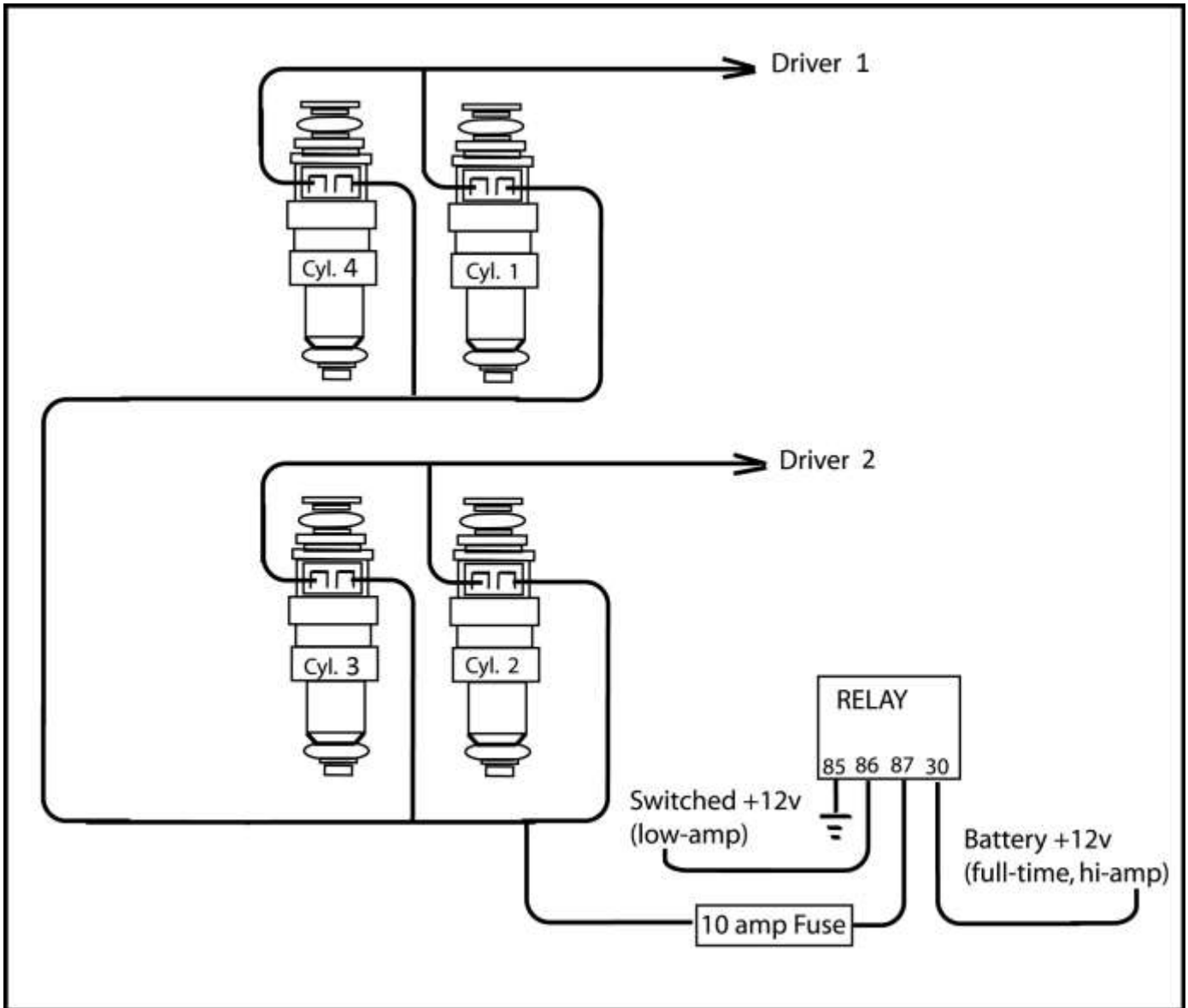
Figure 19. 4-cylinder phased-sequential injection wiring for a 1-3-4-2 firing order.
