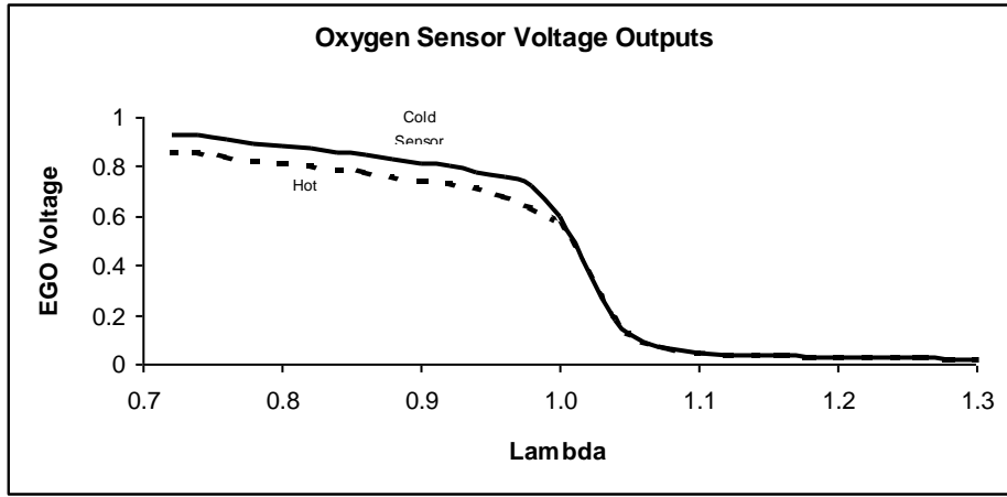
Figure 98: Typical oxygen sensor voltage variation with exhaust temperature.
