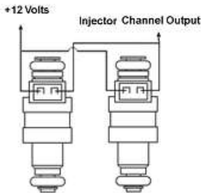
Figure 16: Parallel wiring of fuel injectors. Note that injectors have an electrical polarity. Typically, positive is on the side marked above.
