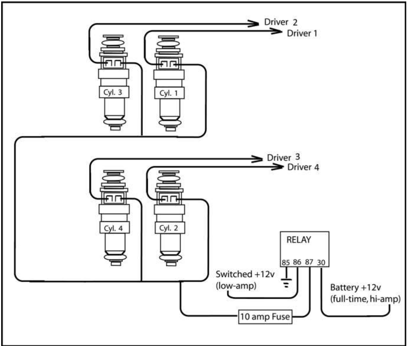
Figure 21. 4-cylinder full-sequential injection wiring for a 1-3-4-2 firing order.
