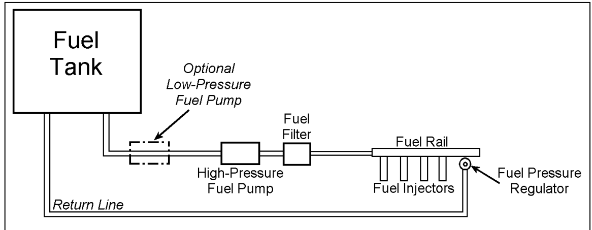
Figure 104: Fuel system plumbing.
