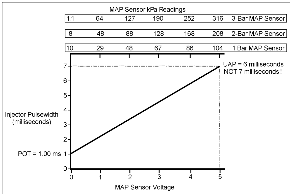
Figure 93: Effect of TOG and IOT on injector pulsewidth. Note: TOG= 6ms , IOT= 1ms .
