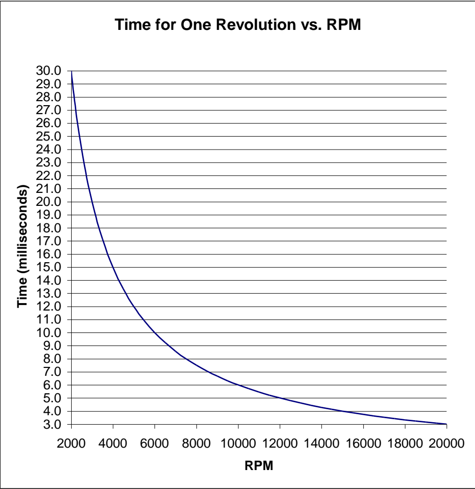
Figure 105: Time between revolutions for various engine speeds.
