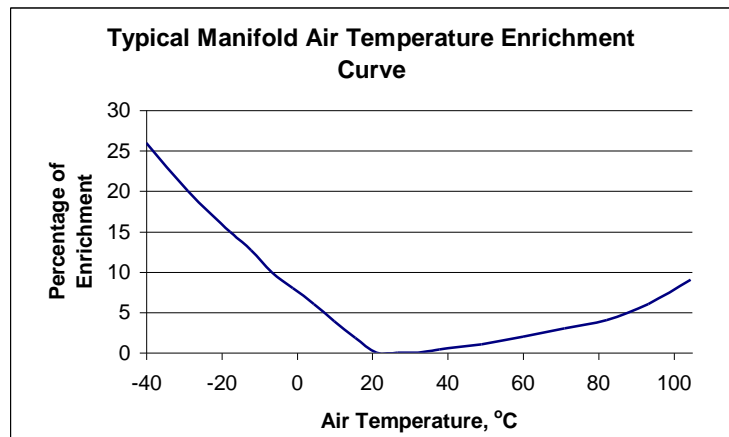
Figure 101: Recommended Starting MAT enrichment curve for turbo-charged applications.
