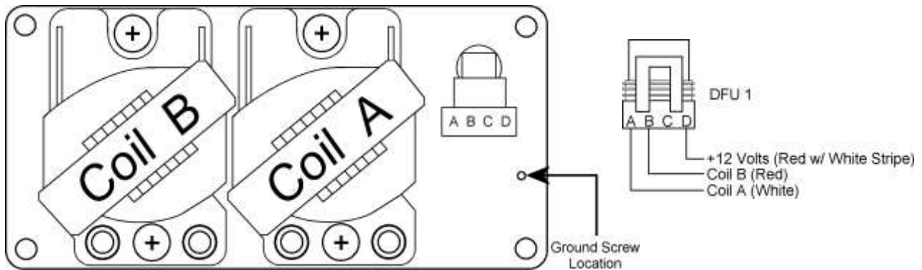
Figure 27. 4-Cyl DFU Setup
