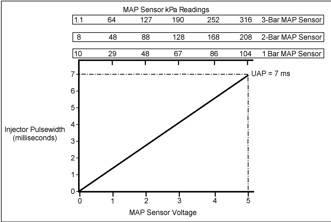
Figure 92: Effect of TOG on injector pulse width. Note: TOG = 7ms , IOT = 0ms .
