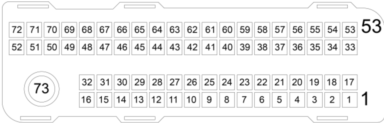
Molex 73 Circuit MX123 Wire Side Shown
