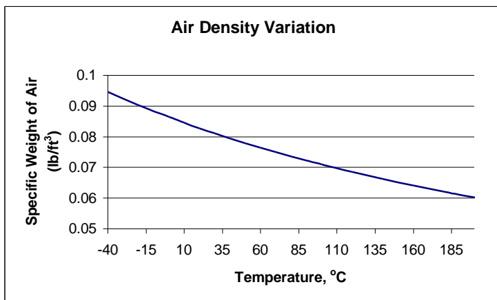
Figure 100: Air Density vs. Temperature
