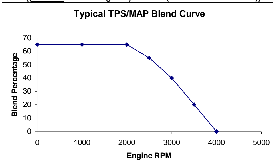
Figure 97: A typical TPS/MAP Blend curve.
