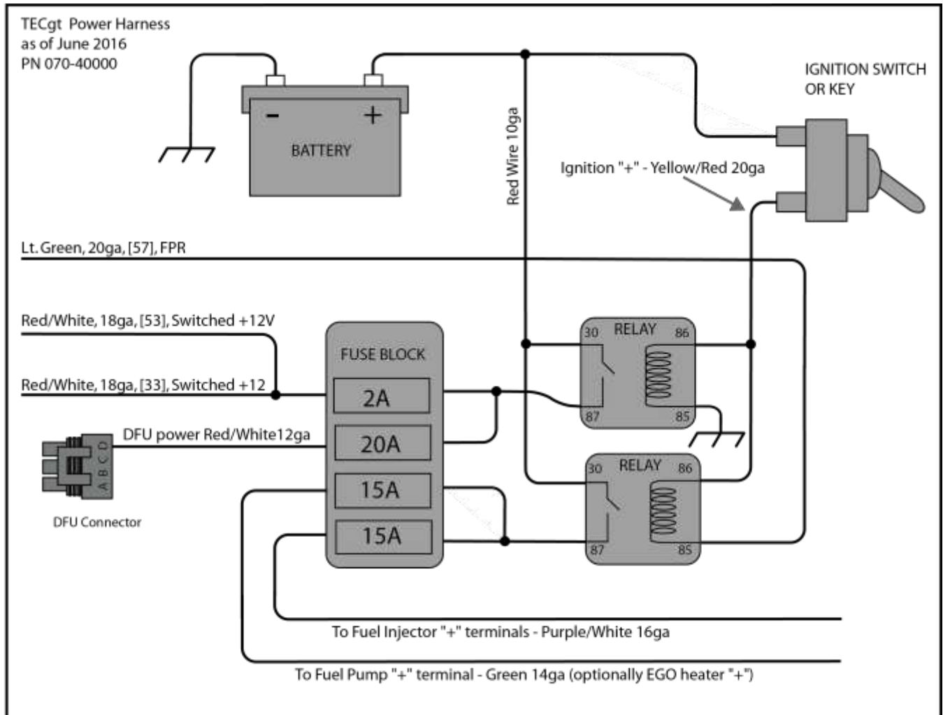
Figure 15. TECs200 Power Harness (PN: 070-40000).
