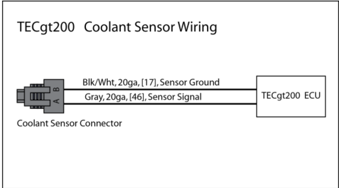
Fig. 51. Coolant temperature sensor wiring.
