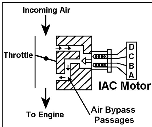
Figure 69: IAC motor plumbing
