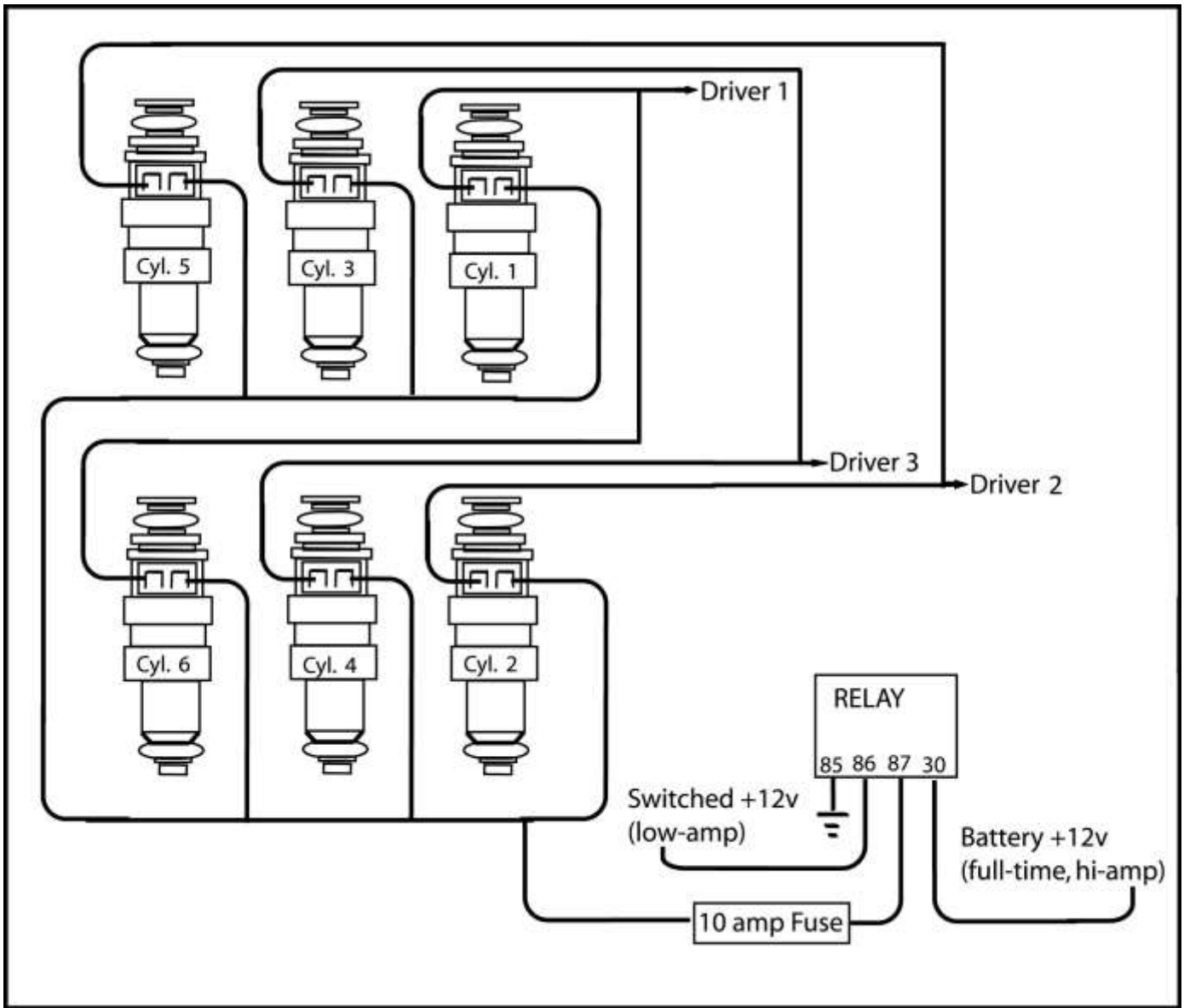
Figure 20. 6-cylinder phased-sequential injection wiring for a 1-5-3-6-2-4 firing order.
