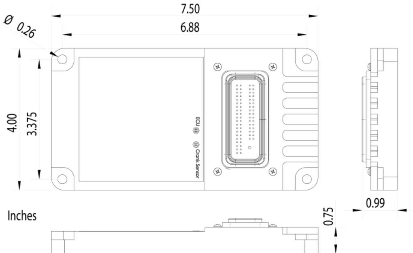
Figure 2. TECs200 ECU
