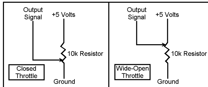
Figure 41 Potentiometer functionality for closed and open throttle conditions.
