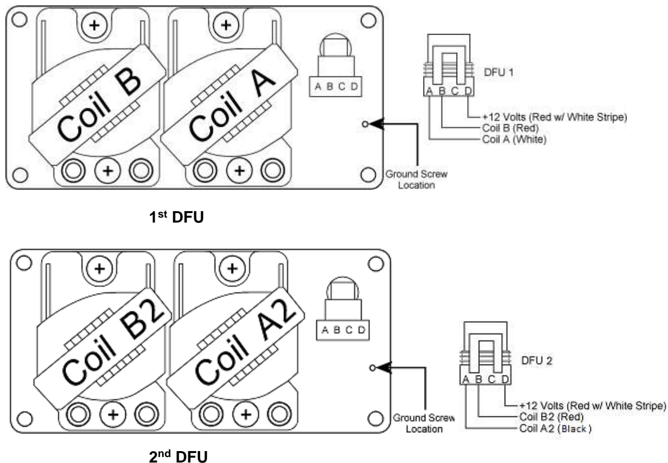
Figure 28: 8-Cyl and 4-cyl Dual Plug DFU Setup. Note that the 2 nd DFU coils will not be labeled C and D from Electromotive. When the 2 nd DFU is wired as shown, the coil labeled “A” will fire coil output “A2.” The coil labeled “B” will fire coil output “B2.”
