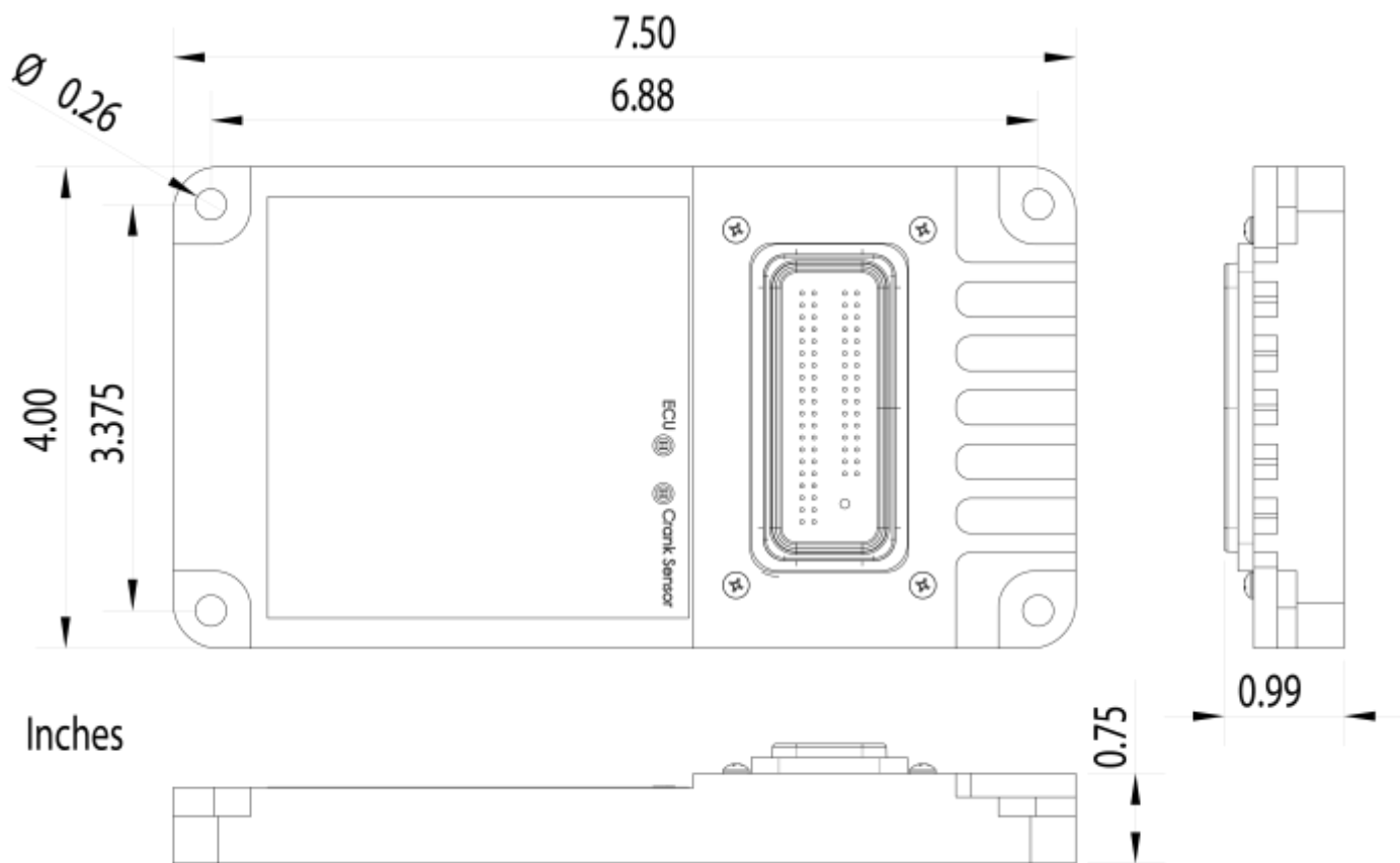
Figure 2. TECgt200 ECU
