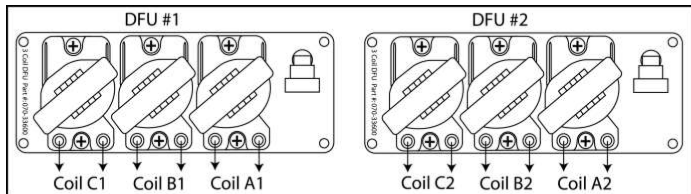
Figure 26 : Coil notation
