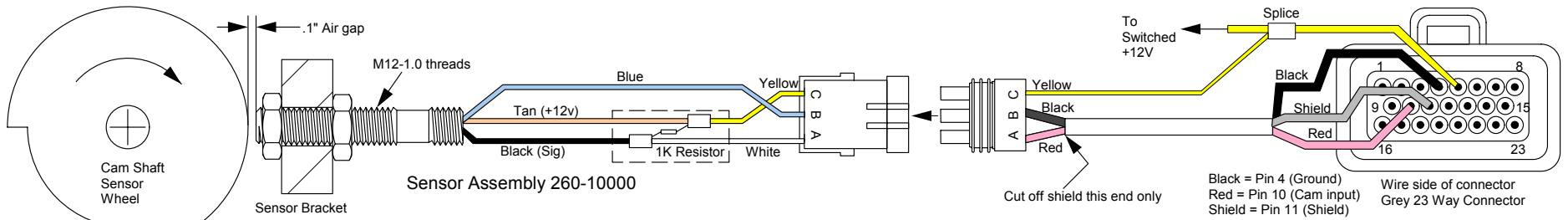
Recommended Hall Effect, Cam Shaft Pickup Installation
