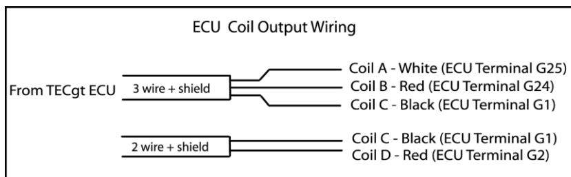
Figure C.1.1: ECU Coil Output Wires (note: shield wire is connected inside the TECgt unit, not connected at the coils).
