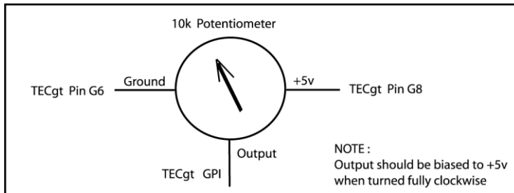
Fig H.1.1: Potentiometer wiring for Fuel, Ignition and GP I/O Trim Inputs
